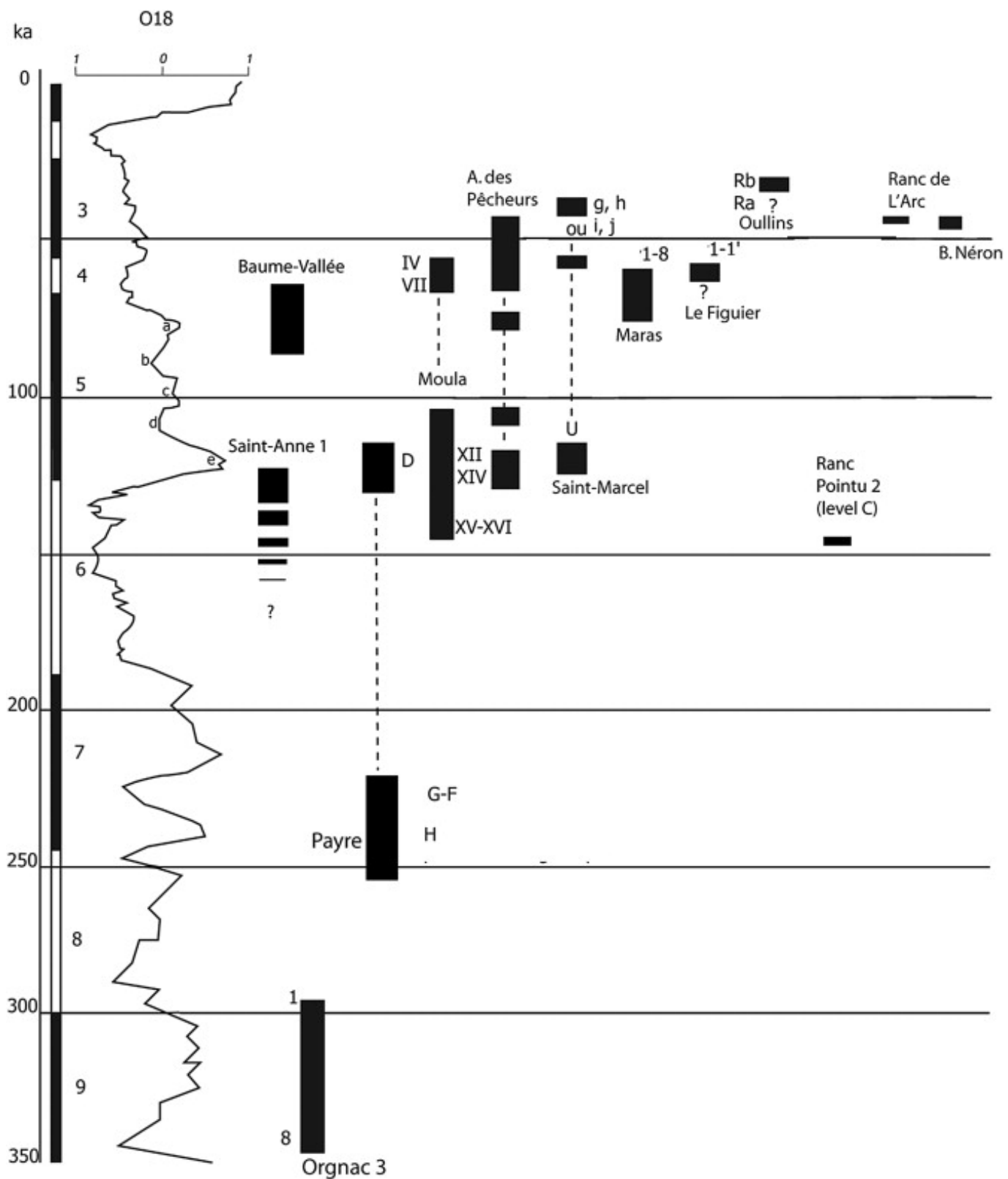
Marine Isotopic Stages, according to Imbrie, 1984
